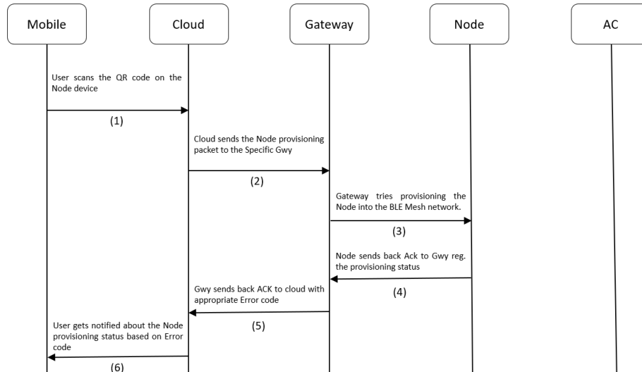
Figure 10.20 Node Provisioning ACK Flow
