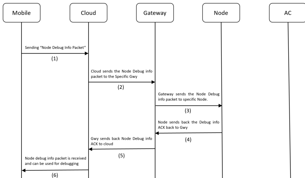
Figure 10.36 Node Debug Info ACK flow
