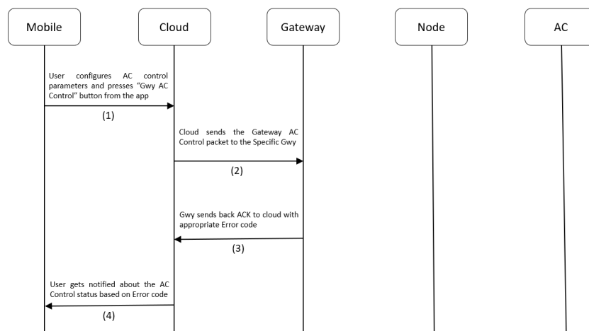
Figure 10.7 Gateway AC Control Process flow
