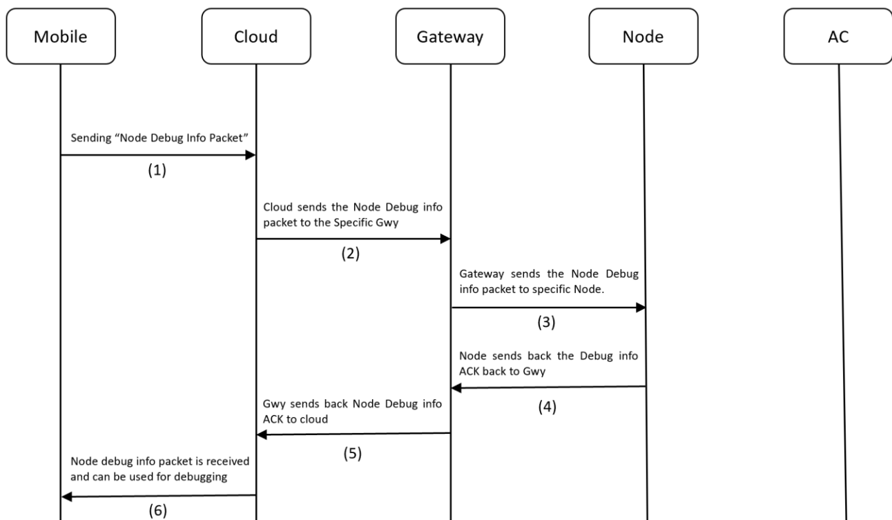
Figure 10.35 Node Debug Info Process Flow
