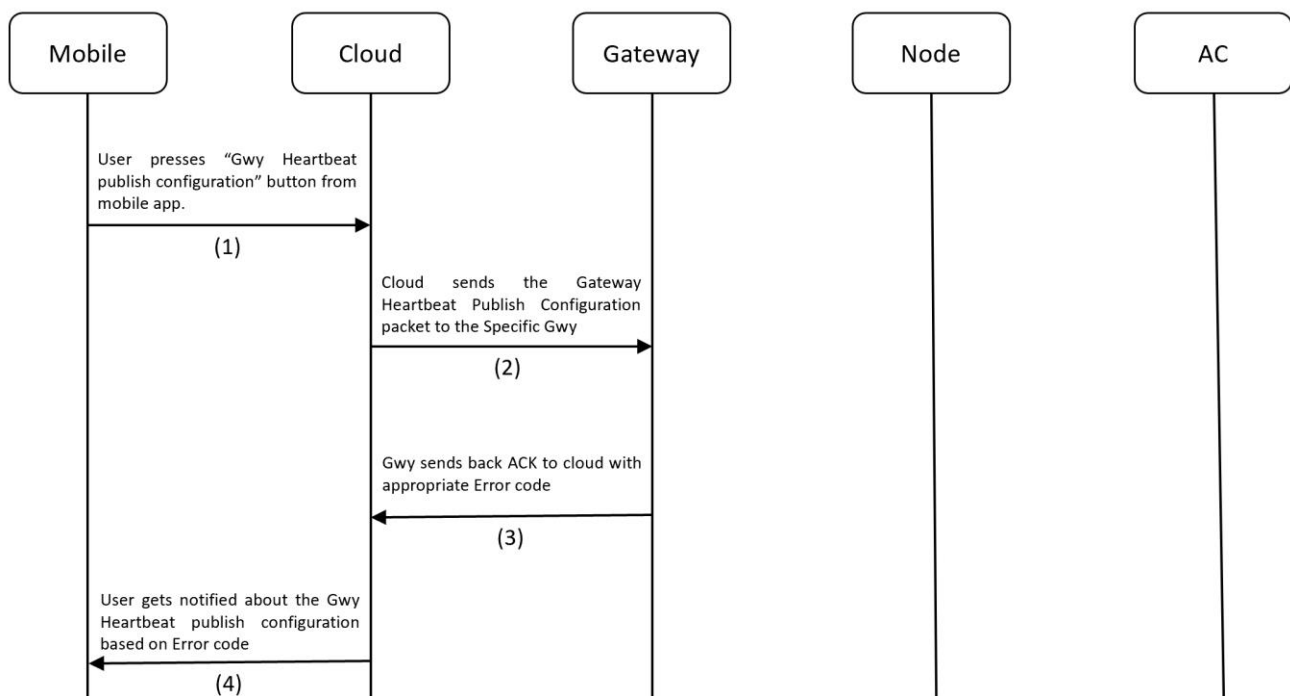
Figure 10.13 Gateway Heartbeat Publish Configuration ACK Process flow
